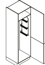
VB Larder - broom unit ↔ 60 ↑ 200 ↙ 60/50
