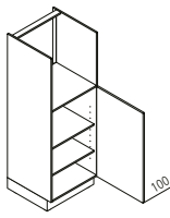
GB Appliance housing for oven or microwave ↔ 60 ↑ 160 ↙ 60
