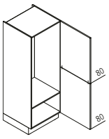
GK Appliance housing for fridge / aperture 123 cm ↔ 60 ↑ 160 ↙ 60
