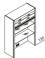
HAJV Top-mounted unit with glass-look louvre door ↔ 50/60/80/90 ↓ 115/130/145 ↱ 35/50/60
