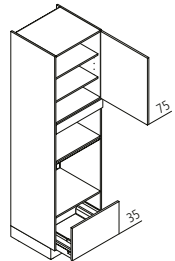
GBBA Appliance housing for oven or microwave ↔ 60 ↑ 215 ↲ 60
