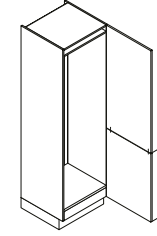
GK Appliance housing for fridge / aperture 178 cm ↔ 60 ↑ 200 ↙ 60
