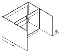
SOD Sink base unit ↔ 80/90/100/120 ↑ 80 ↘ 60
