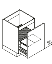
SABD Sink base unit with waste separation system ↔ 45/50/60 ↑ 80 ↘ 60
