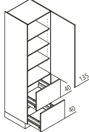
VZ Larder unit ↔ 30/40/45/50/60 ↑ 215 ↲ 60/50
