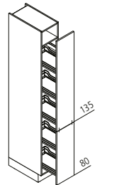
VVA Larder unit ↔ 30/40 ↑ 215 ↲ 60
