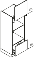
GBLA Appliance housing with lift-up door for microwave and oven ↔ 60 ↑ 160 ↙ 60
