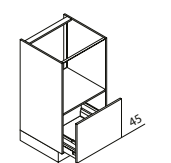
GBZ Appliance housing for oven or microwave ↔ 60 ↓ 105 ↱ 60
