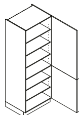
VT Larder unit ↔ 30/40/45/50/60 ↑ 200 ↙ 60/50/39
